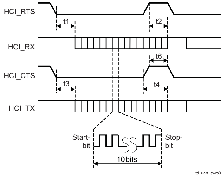
Figure 5-1. UART Timing
